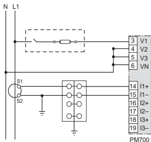
Figure 4-1: 1-Phase Line-to-Neutral 2-Wire System 1 CT
