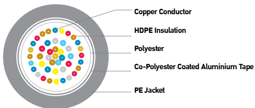
OUTDOOR CAT 3 UTP Cable
