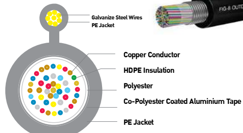
FIG-8 OUTDOOR CAT 3 UTP Cable
