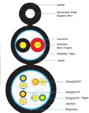
US-9015M CAT 5E UTP, PE OUTDOOR w/Drop Wire (Single Jacket)
